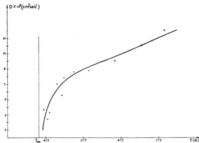
Fig. 1. Self-diffusion coefficient of tin in the liquid Sn–Pb eutectic alloy as a function of temperature.
